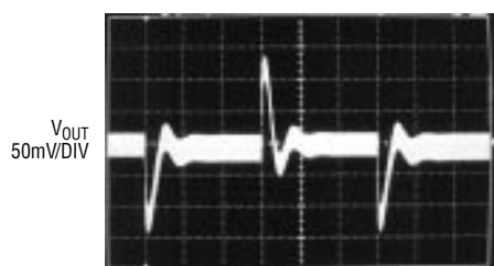
Transient Response
