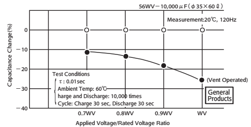
Fig-24 Rapid charge and discharge characteristics (Effects of Applied Voltage)
