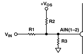
Figure 16. Scaling and Offsetting A_{IN(1-2)} for Bipolar Inputs
