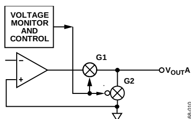
Figure 42. Analog Output Control Circuitry
