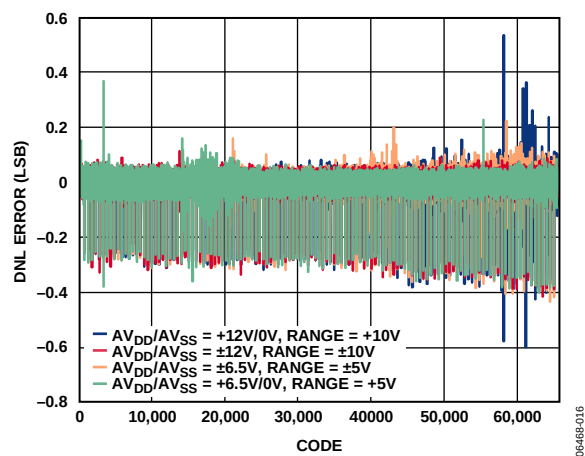
Figure 9. AD5754 Differential Nonlinearity Error vs. Code
