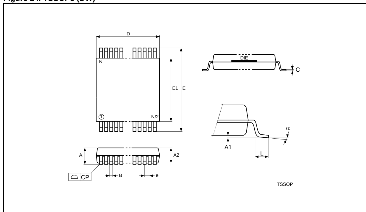
Figure 14. TSSOP8 (DW)
