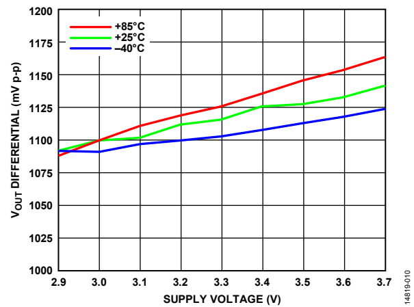
Figure 11. Output ( V_{OUT} ) Differential vs. Supply Voltage, VR = 3.3 V, Frequency = 13 GHz
