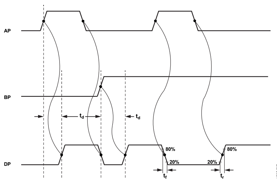
Figure 17. Timing Diagram
