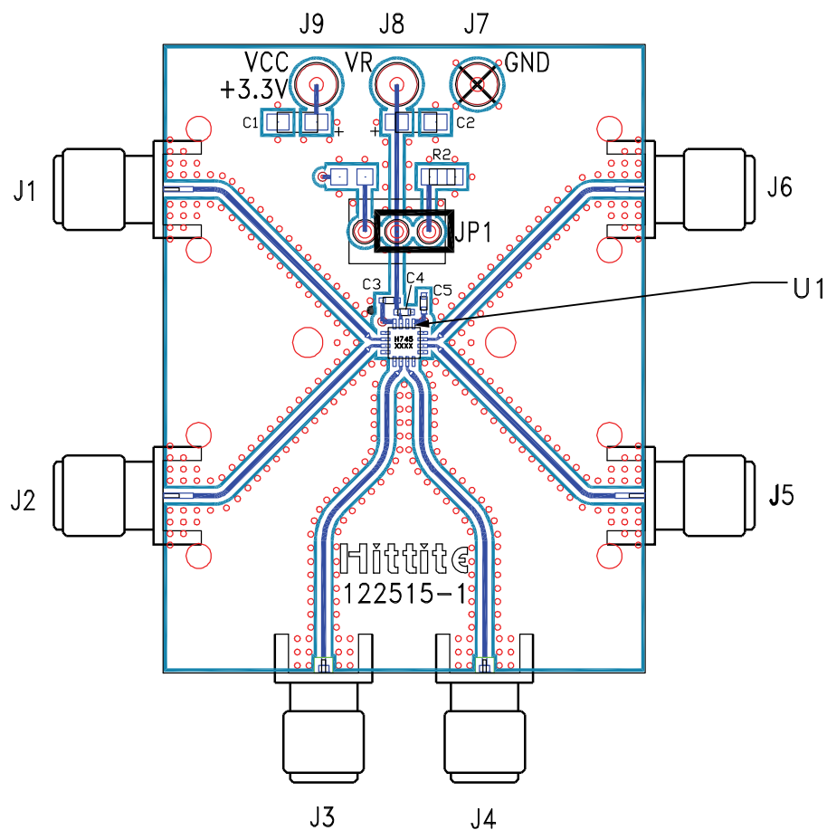
Figure 18. Evaluation Board
