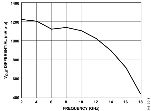
Figure 12. Output ( V_{OUT} ) Differential vs. Frequency, VR = 3.3 V
