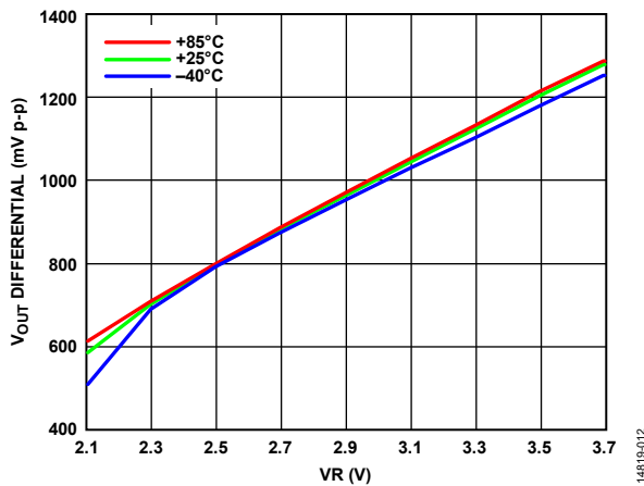
Figure 10. Output ( V_{OUT} ) Differential vs. VR, Frequency = 13 GHz
