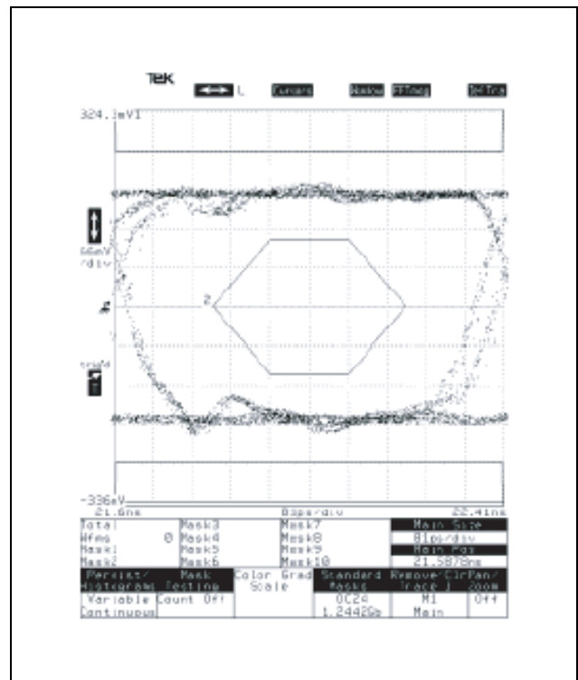
Figure 6 P_{\text{opt}} = 500 \mu\text{W avg. (OC-24)}
