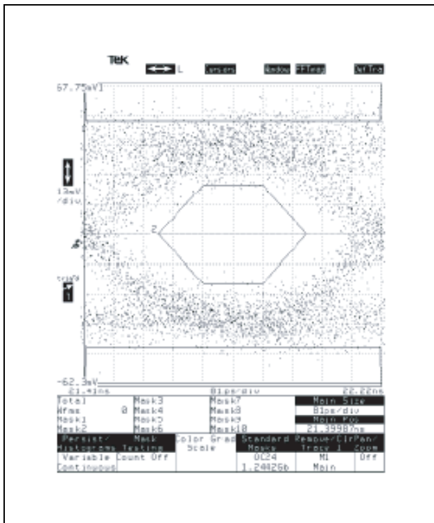
Figure 3 P_{\text{opt}} = 2 \mu\text{W avg. (OC-24)}
