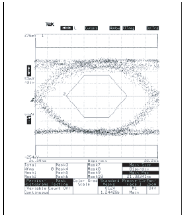
Figure 5 P_{\text{opt}} = 10 \mu\text{W avg. (OC-24)}
