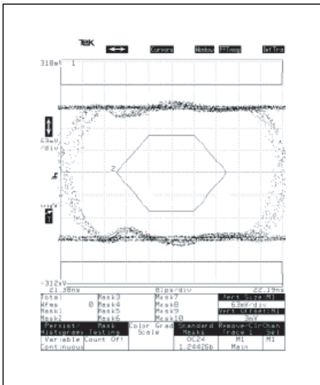
Figure 4 P_{\text{opt}} = 100 \mu\text{W avg. (OC-24)}
