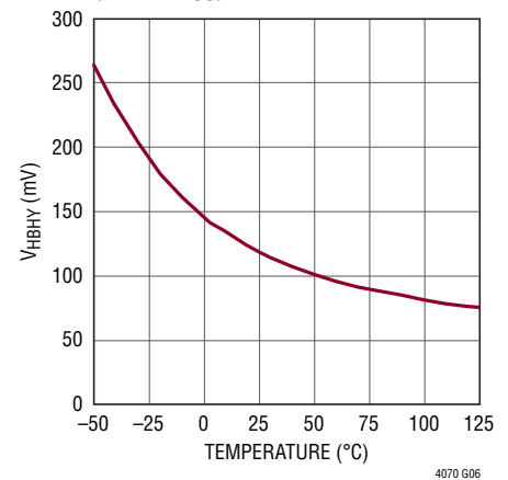
V_{HBHY} vs Temperature (ADJ = V_{CC} )
