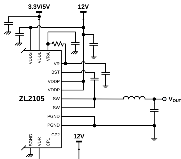
Figure 12. Dual Input Supply Operation
