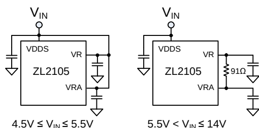
Figure 8. Input Supply Connections
