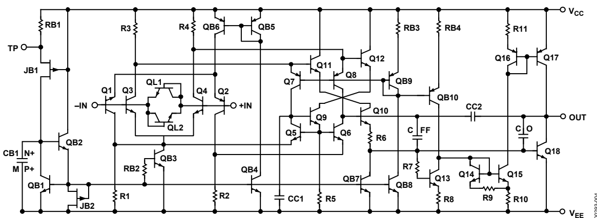
Figure 4. Simplified Schematic
