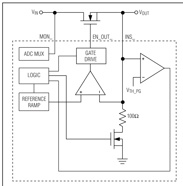
Figure 16. Closed-Loop Tracking
