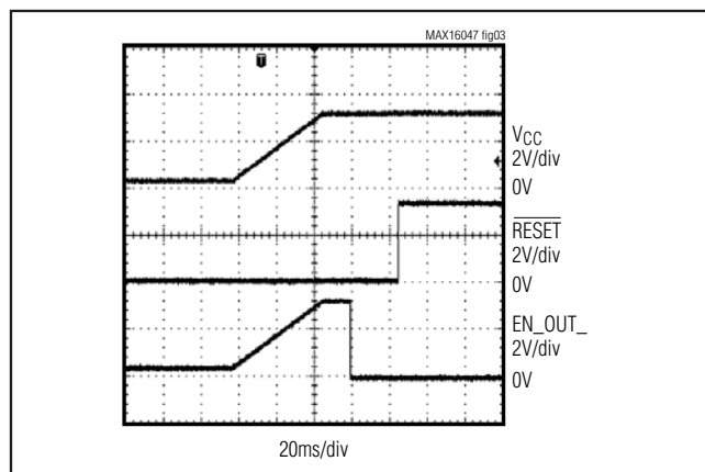
Figure 3. \overline{\text{RESET}} and EN_OUT_ During Power-Up, EN_OUT_ Is in Open-Drain Active-Low Configuration
