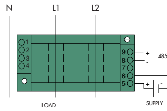
CRD4150 Single Element, 3-Wire
