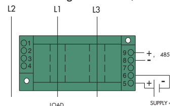
CRD4150 3 Element, 3-Wire
