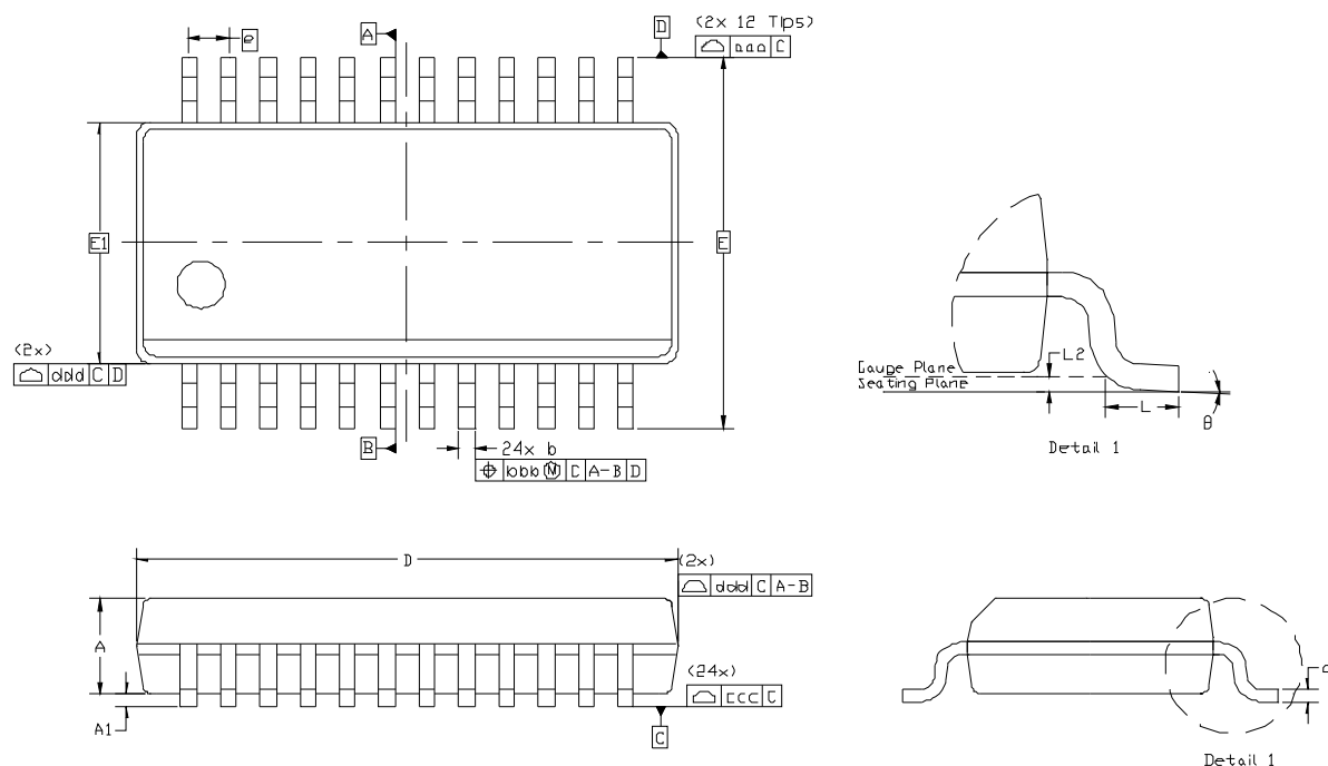
Figure 3.8. QSOP-24 Package Diagram
