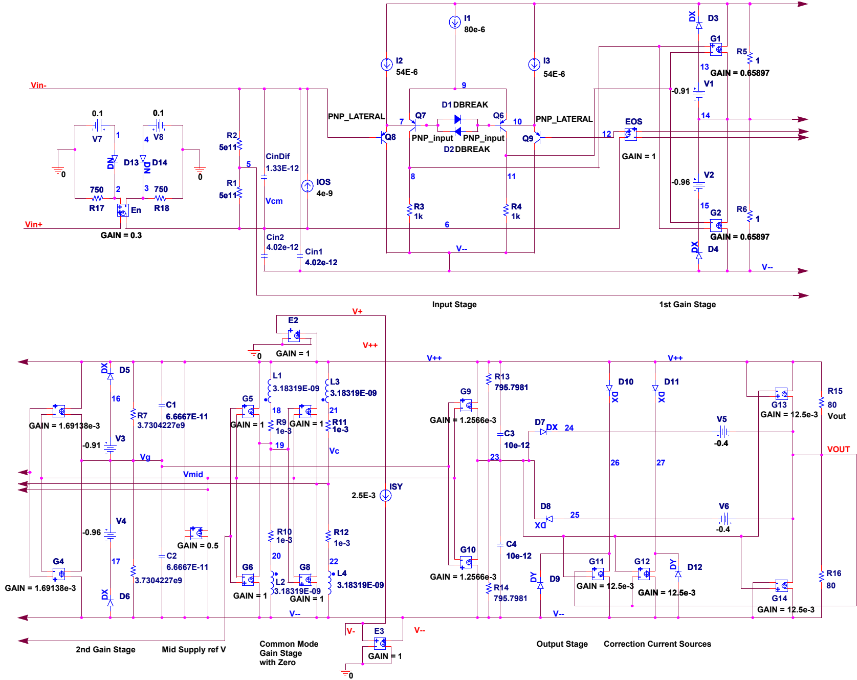
FIGURE 50. SPICE SCHEMATIC
