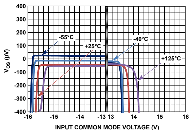
FIGURE 6. INPUT OFFSET VOLTAGE vs INPUT COMMON MODE VOLTAGE, -55^{\circ}C to +125^{\circ}C , V_S = \pm 15V
