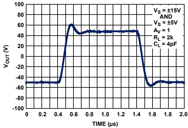
FIGURE 64. CHARACTERIZED SMALL-SIGNAL TRANSIENT RESPONSE
