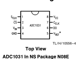
Dual-In-Line and SO Packages
