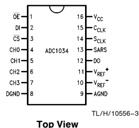
Dual-In-Line and SO Packages
