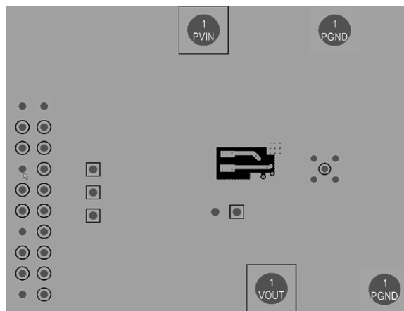
Figure 8. Mid-Layer 2
