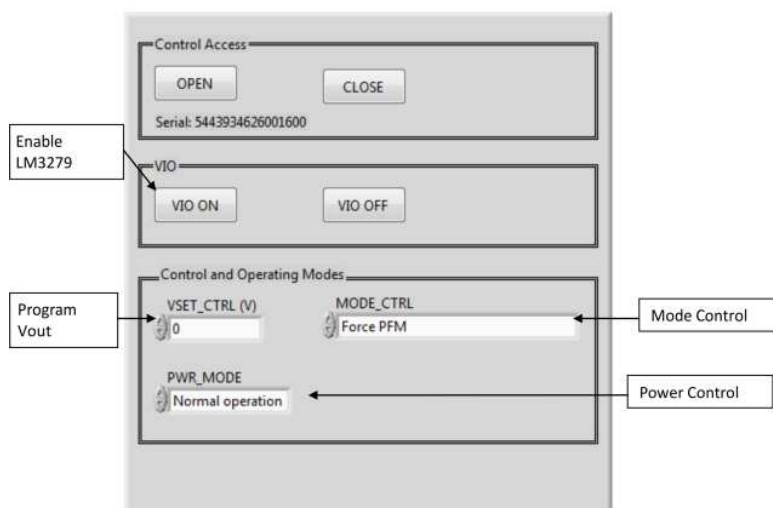
Figure 11. Programming GUI Window
