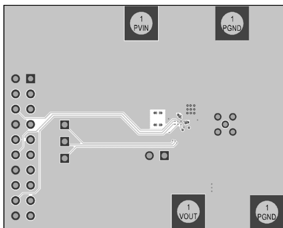
Figure 7. Mid-Layer 1
