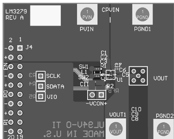
Figure 6. Top Layer 1
