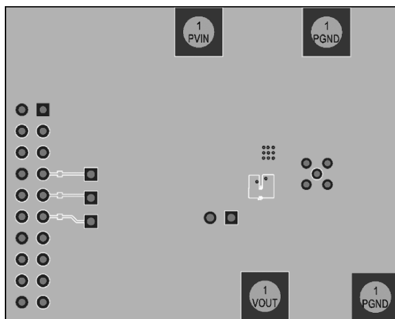
Figure 9. Bottom Layer
