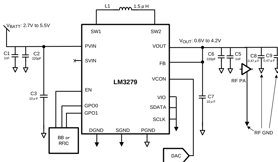
Figure 2. Analog Circuit
