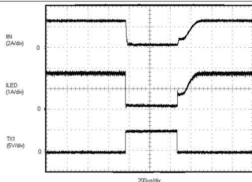
Figure 21. AET-Mode Operation
