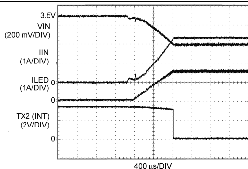
Figure 19. V_{IN} Flash Monitor Operation
