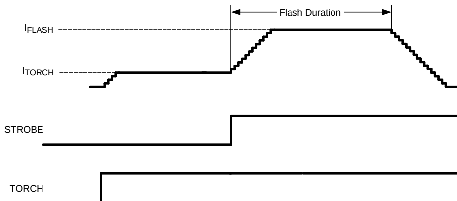
Figure 26. Hardware-Torch Mode
