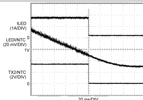
Figure 20. NTC-Mode Operation
