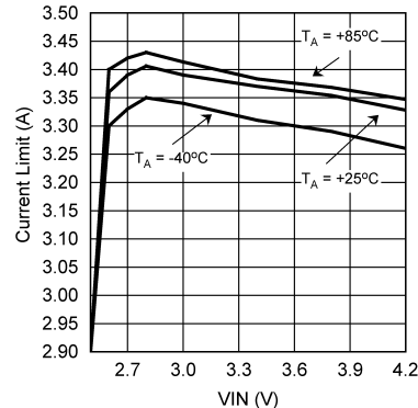
Figure 2. Closed Loop Current Limit vs V_{IN} Flash Duration
