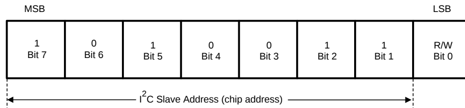
Figure 41. Device Address
