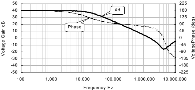
Bch Voltage Gain , Phase vs. Frequency Characteristic ( V+=5V ,Ta=25°C )
