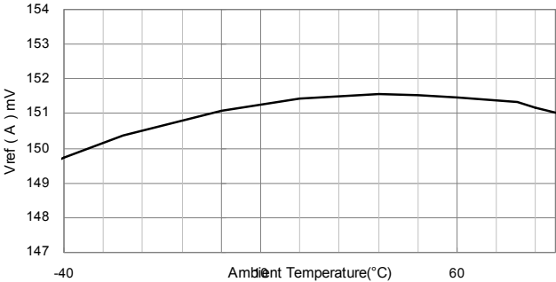
VOLTAGE REFERENCE (C Version)
