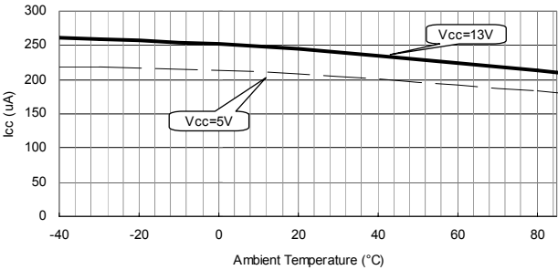
Supply Current(Icc) vs. Temperature
