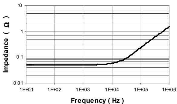
Impedance v. Frequency
