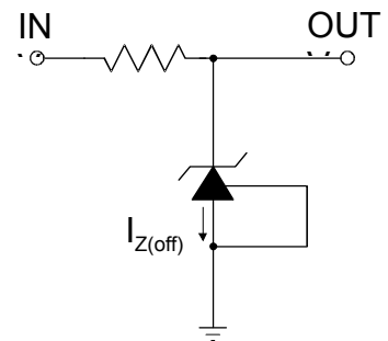
Test Circuit 3
