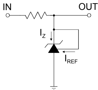
Test Circuit 1
