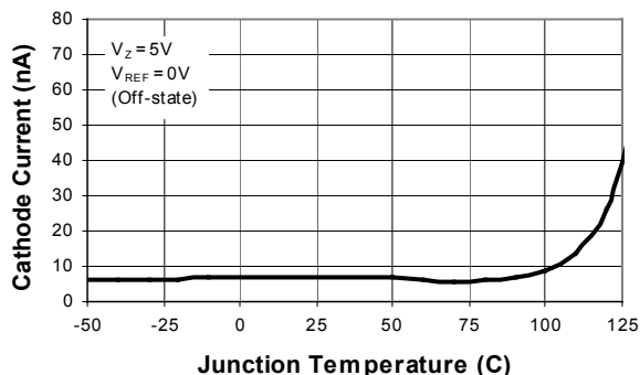
Cathode Current v. Temperature
