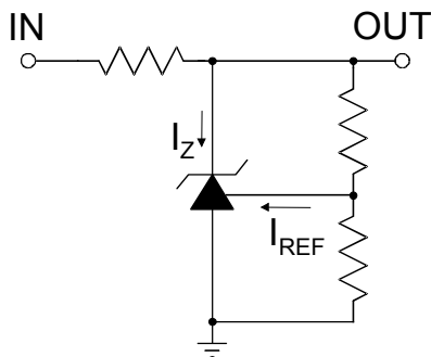
Test Circuit 2
