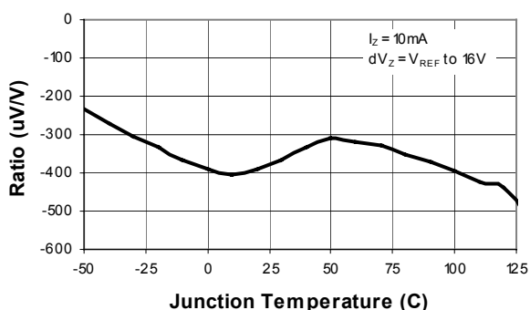
Ratio of \Delta V_{REF} / \Delta V_Z v. Temperature
