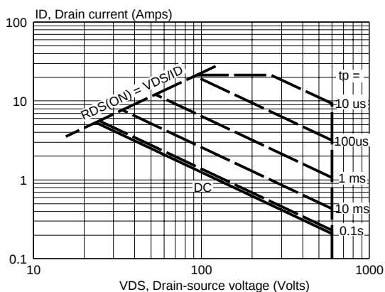
Fig.3. Safe operating area. T_{mb} = 25\ ^\circ C I_D \text{ \& } I_{DM} = f(V_{DS}); I_{DM} \text{ single pulse; parameter } t_p
