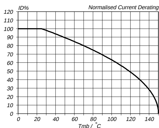
Fig.2. Normalised continuous drain current. ID\% = 100 \cdot I_D / I_{D\ 25\ ^\circ C} = f(T_{mb}); \text{ conditions: } V_{GS} \geq 10\ V
