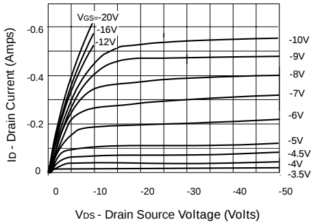
Output Characteristics
