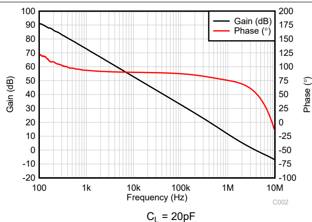
Figure 4-10. Open-Loop Gain and Phase vs Frequency
