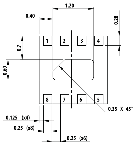
BOTTOM VIEW
