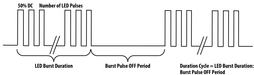
Figure 3. LEDA Burst Pulses Definition
