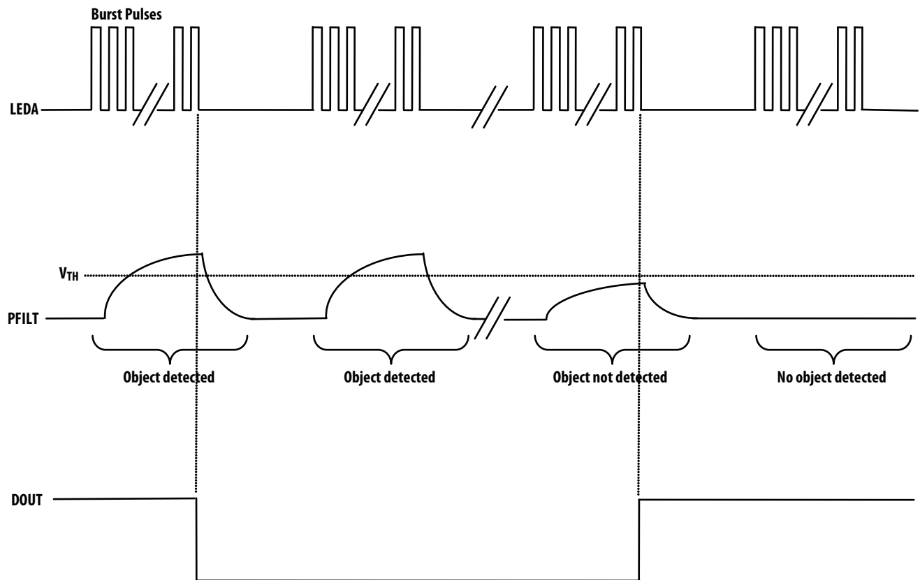
Figure 4. Output Waveforms Definition
