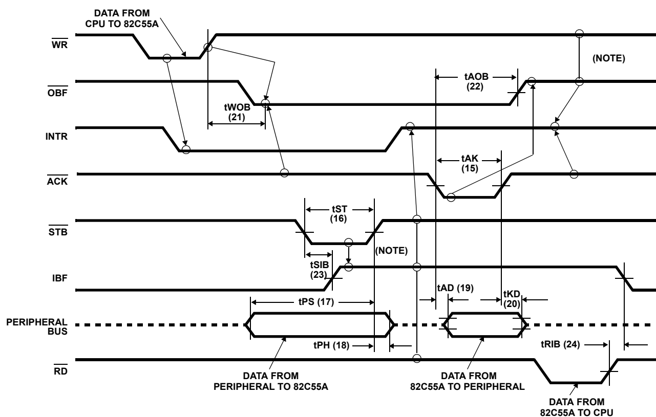
FIGURE 29. MODE 2 (BIDIRECTIONAL)
