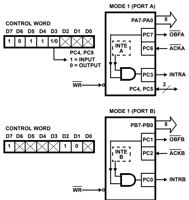
FIGURE 8. MODE 1 OUTPUT
