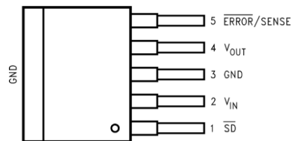
Figure 2. 5-Pin DDPAK/TO-263 (Top View) See KTT Package
