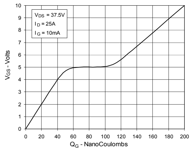
Fig. 10. Gate Charge
