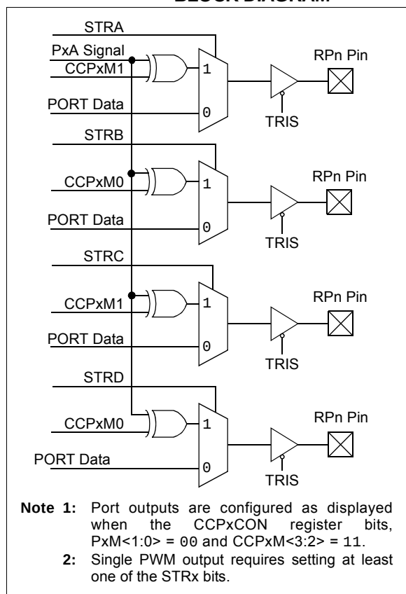
FIGURE 18-18: SIMPLIFIED STEERING BLOCK DIAGRAM
