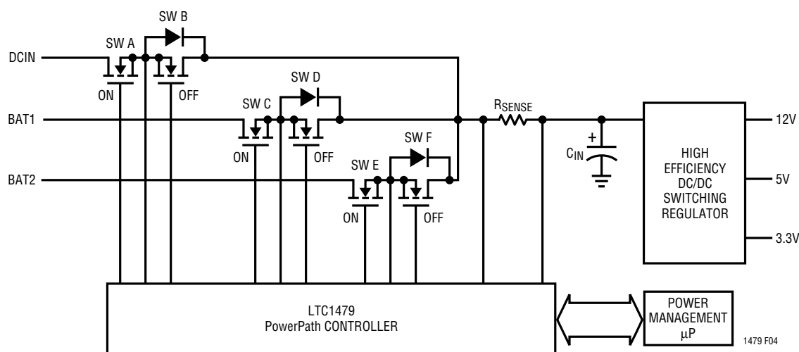
Figure 4. LTC1479 PowerPath Switches in “3-Diode” Mode
