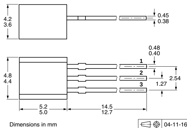
Fig 12. Package outline SOT54 (SC-43A/TO-92)
