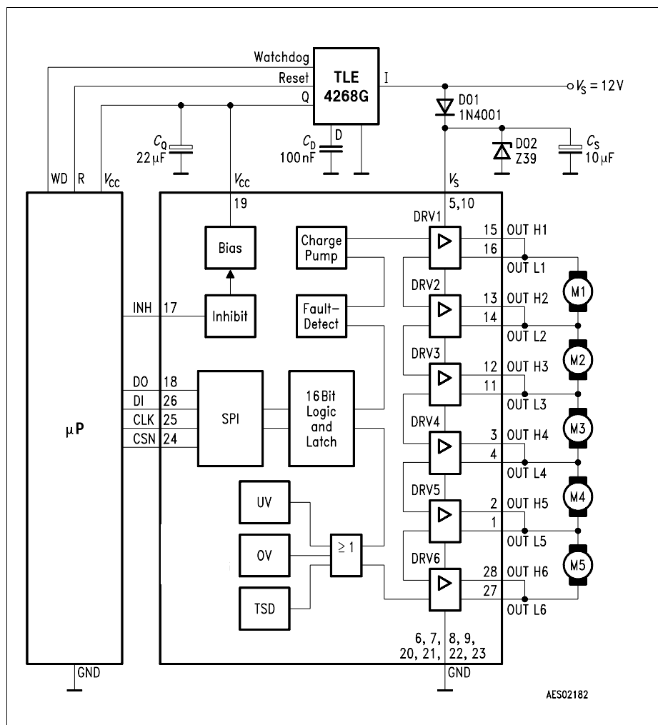
Figure 10 Application Circuit
