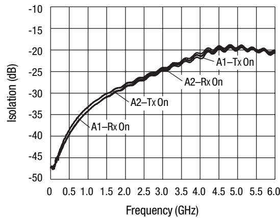
A1-A2 Isolation
