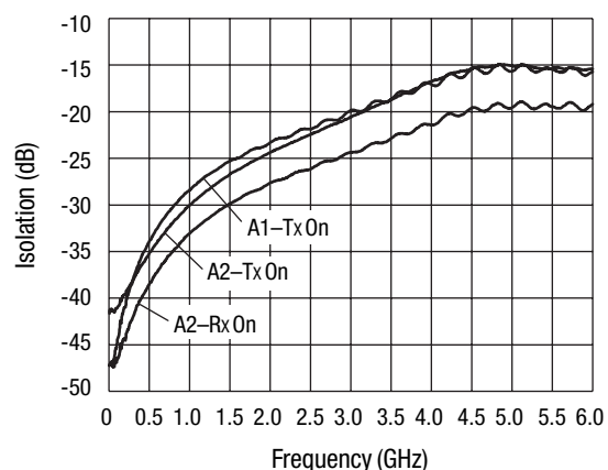
A1-Rx Isolation
