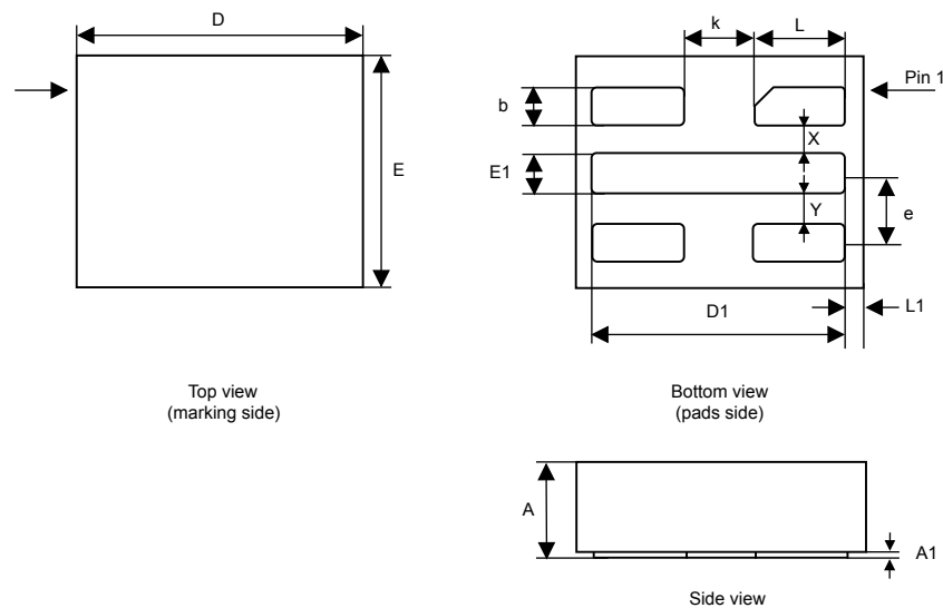
Figure 30. UFDFPN5 - Outline
