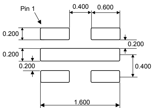
Figure 31. UFDFPN5 - Footprint example
