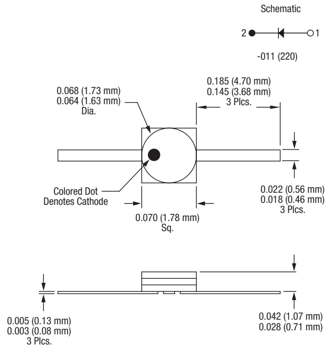
Figure 5. -220 Package Dimensions
