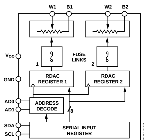
Figure 2. AD5173
