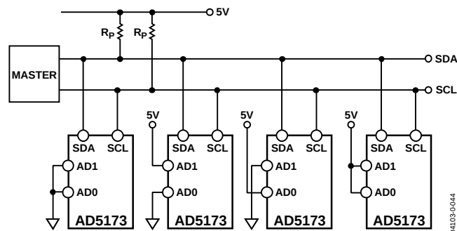
Figure 54. Multiple AD5173s on One I 2 C Bus
