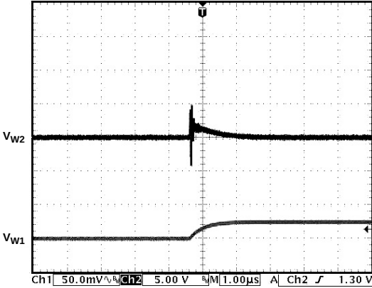
Figure 24. Analog Crosstalk
