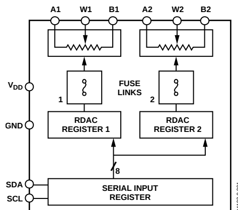
Figure 1. AD5172
