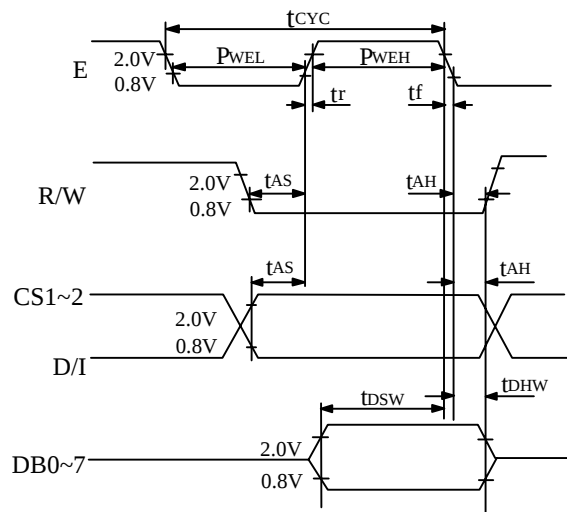
Fig . 1 CPU Write Timing
