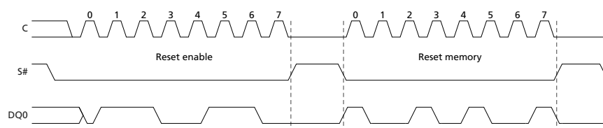
Figure 35: Serial Input Timing
