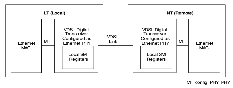
Figure 21 PHY-PHY Scenario
