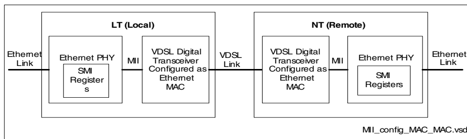
Figure 20 MAC-MAC Scenario
