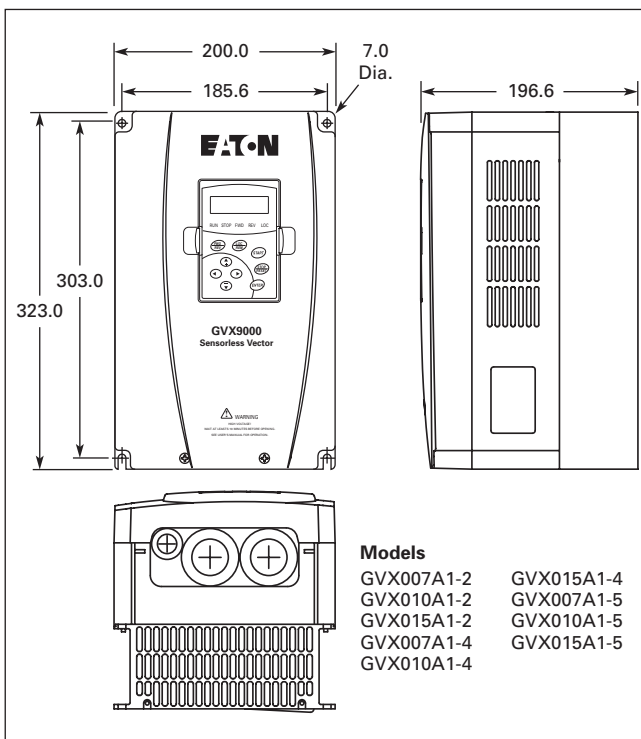
Figure 4. 5.5 – 11 kW — Approximate Dimensions in mm
