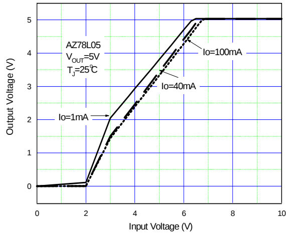
Figure 4. Dropout Characteristics
