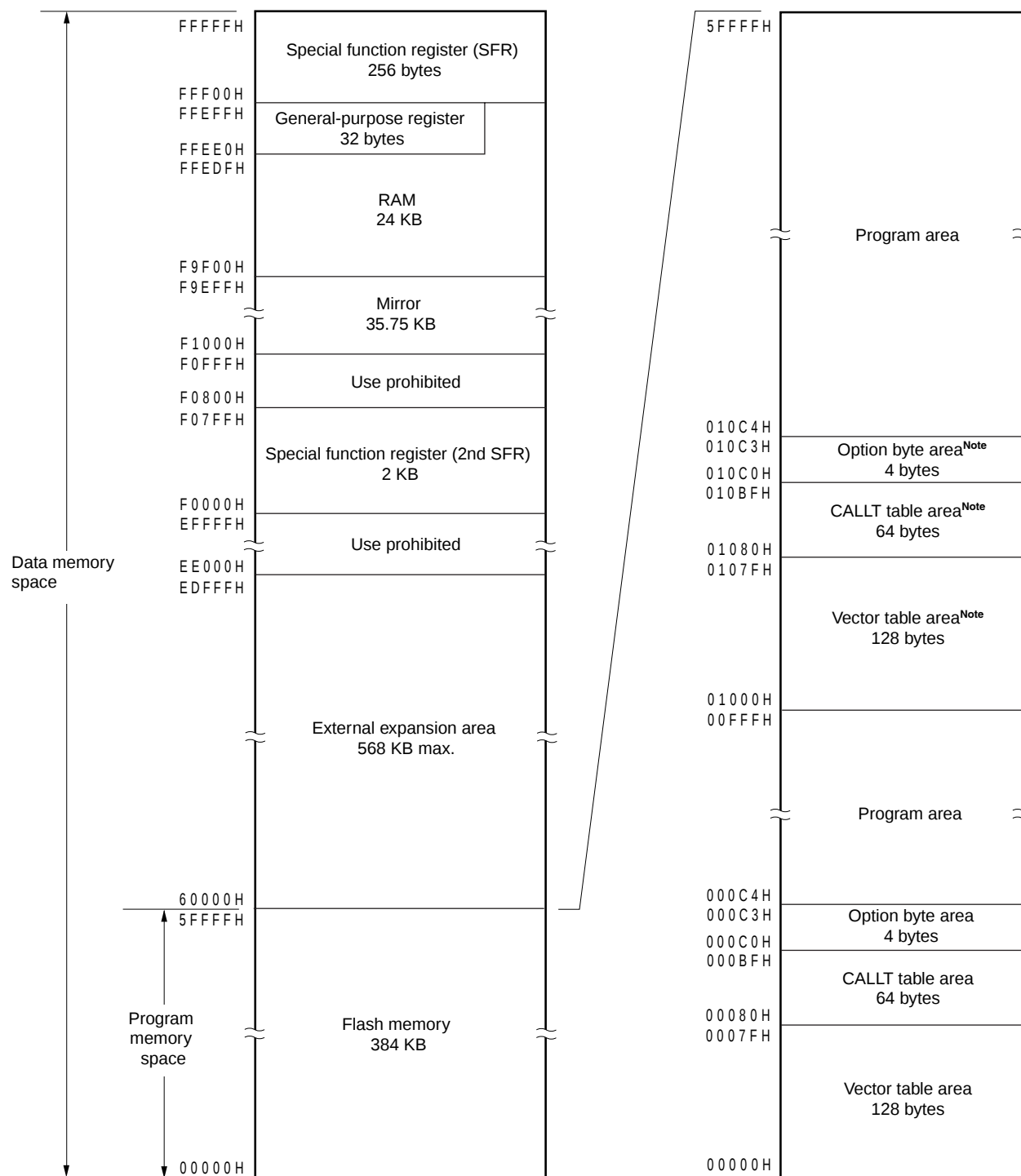
Figure 4-6. Memory Map ( \mu PD78F1167)
