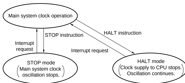
Figure 9-1. Standby Function
