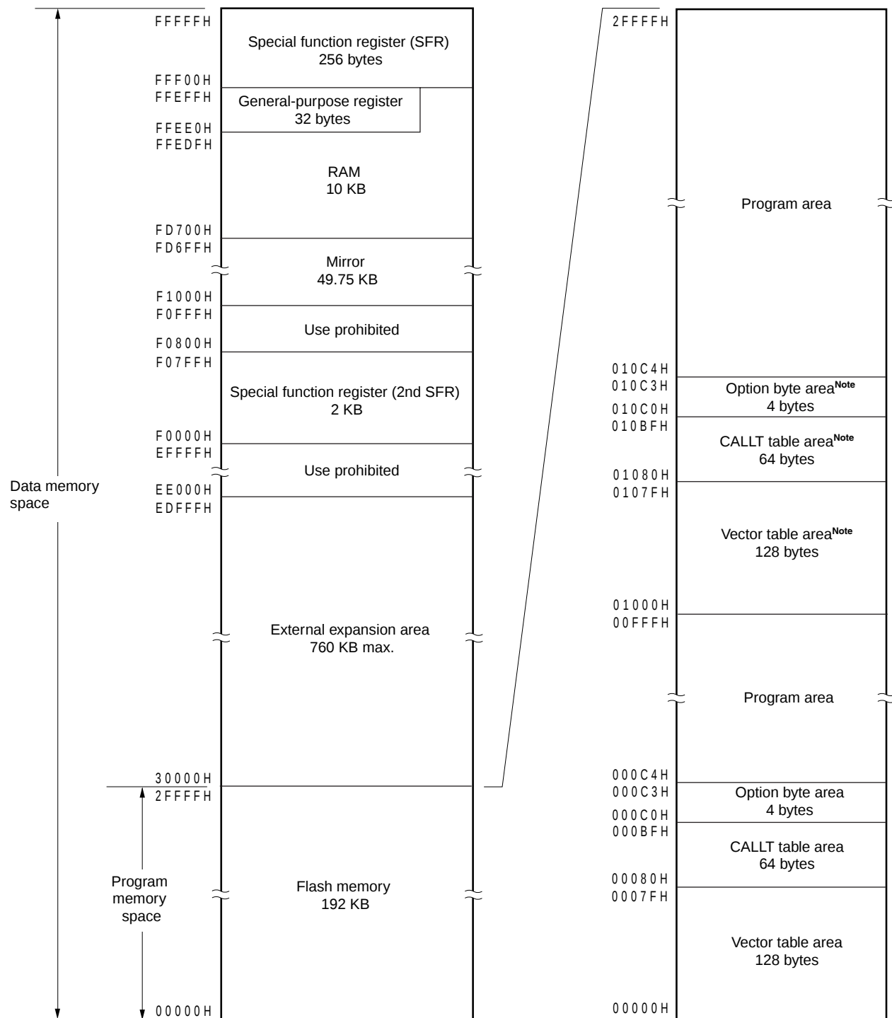
Figure 4-4. Memory Map (μPD78F1165)
