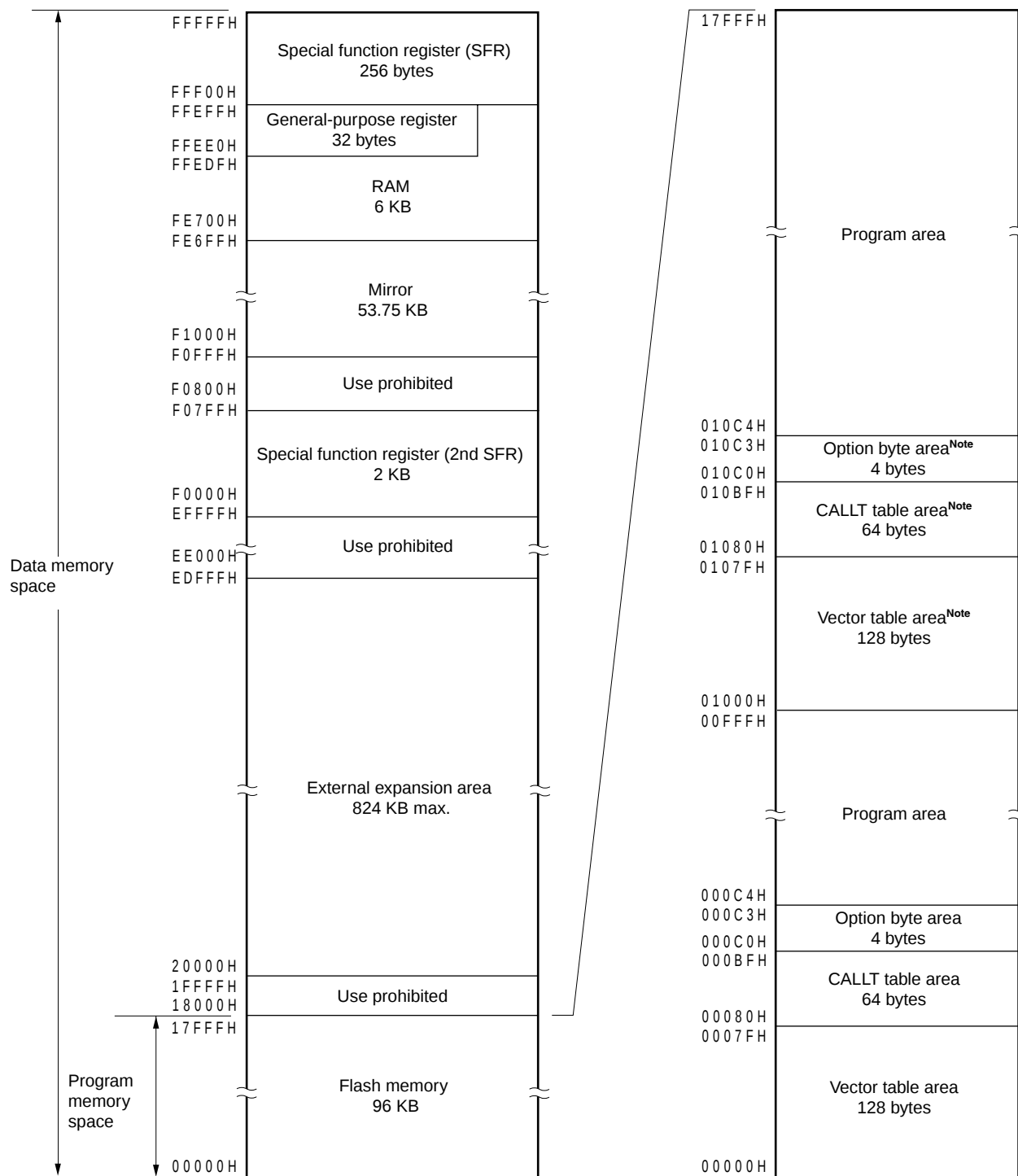
Figure 4-2. Memory Map (μPD78F1163)
