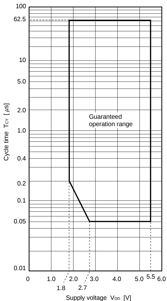
T_{CY} vs. V_{DD} (Main System Clock Operation)
