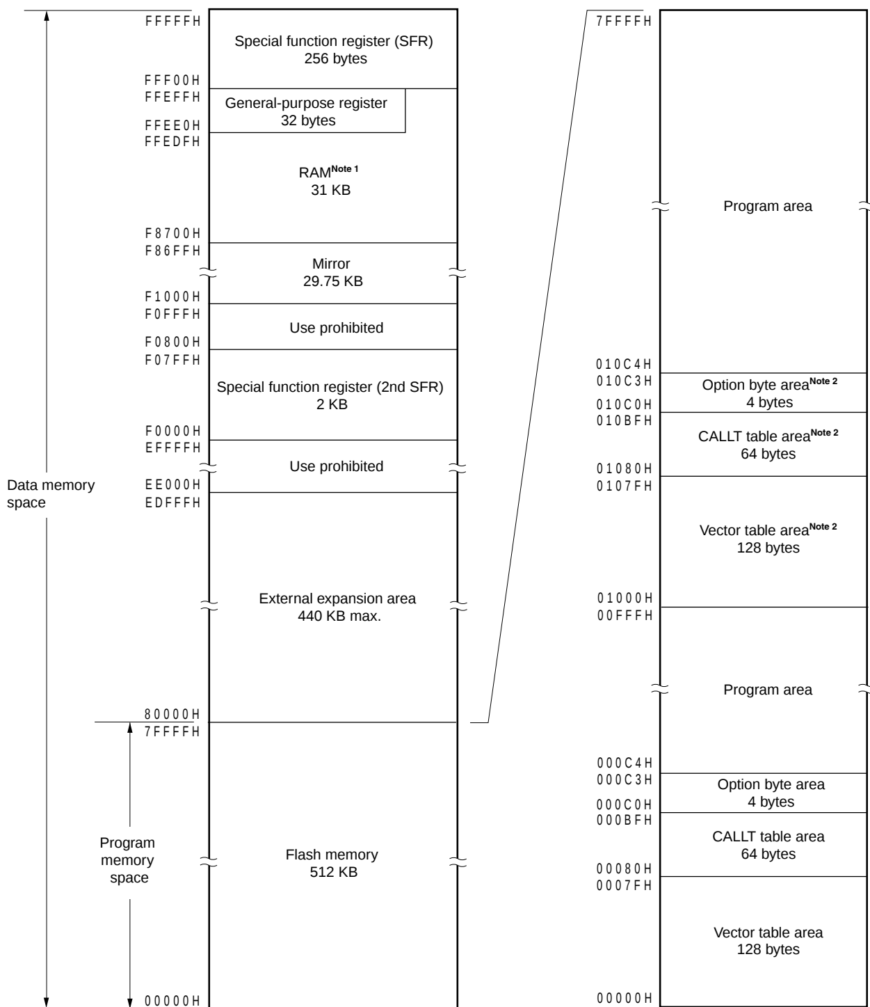
Figure 4-7. Memory Map (μPD78F1168)
