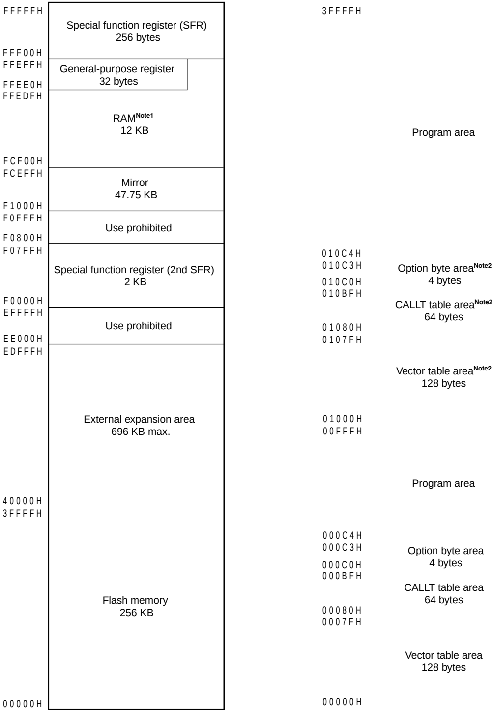
Figure 4-5. Memory Map (μPD78F1166)
