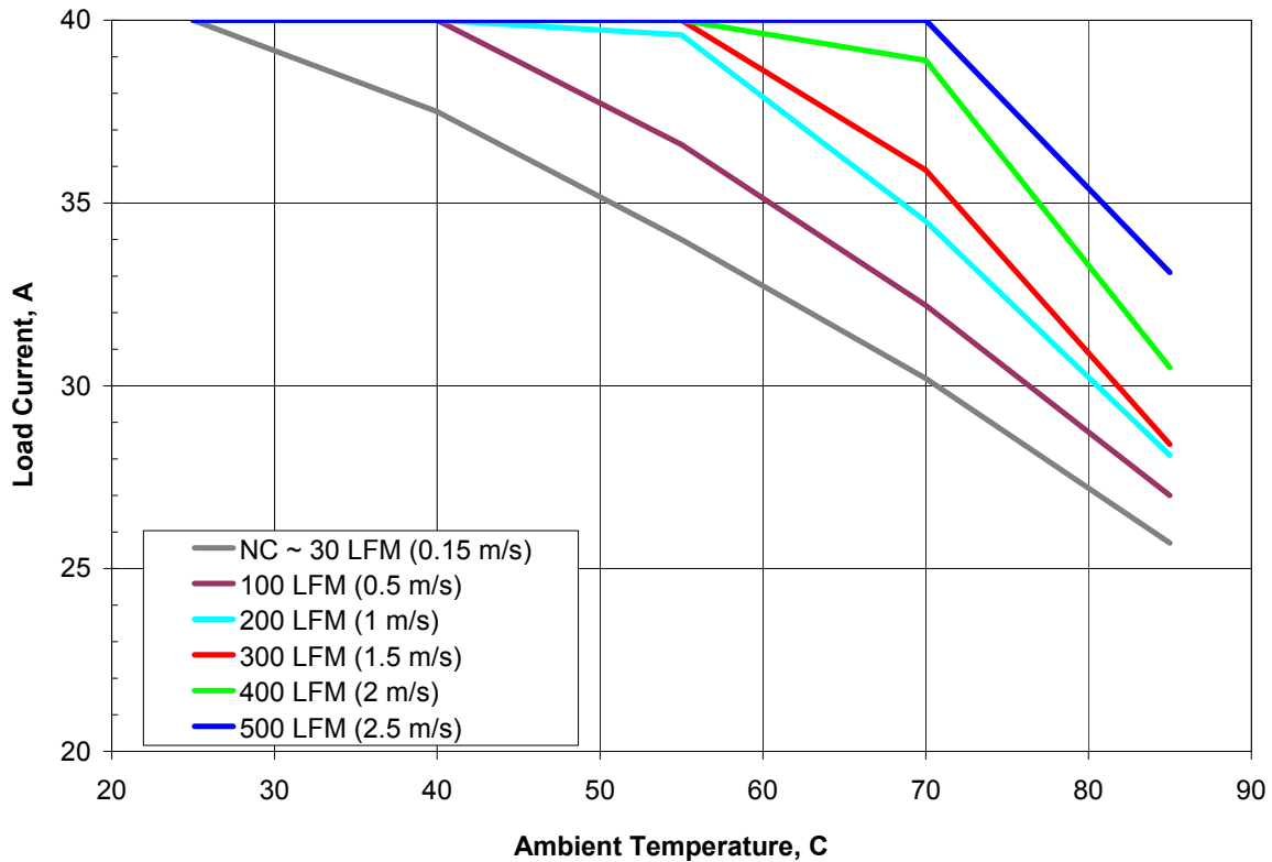
Figure 1. Available load current vs. ambient air temperature and airflow rates for SQE48T40018 converter mounted vertically with air flowing from pin 3 to pin 1, MOSFET temperature \leq 120^{\circ}\text{C} , V_{in} = 48\text{ V} . Note: NC – Natural convection
