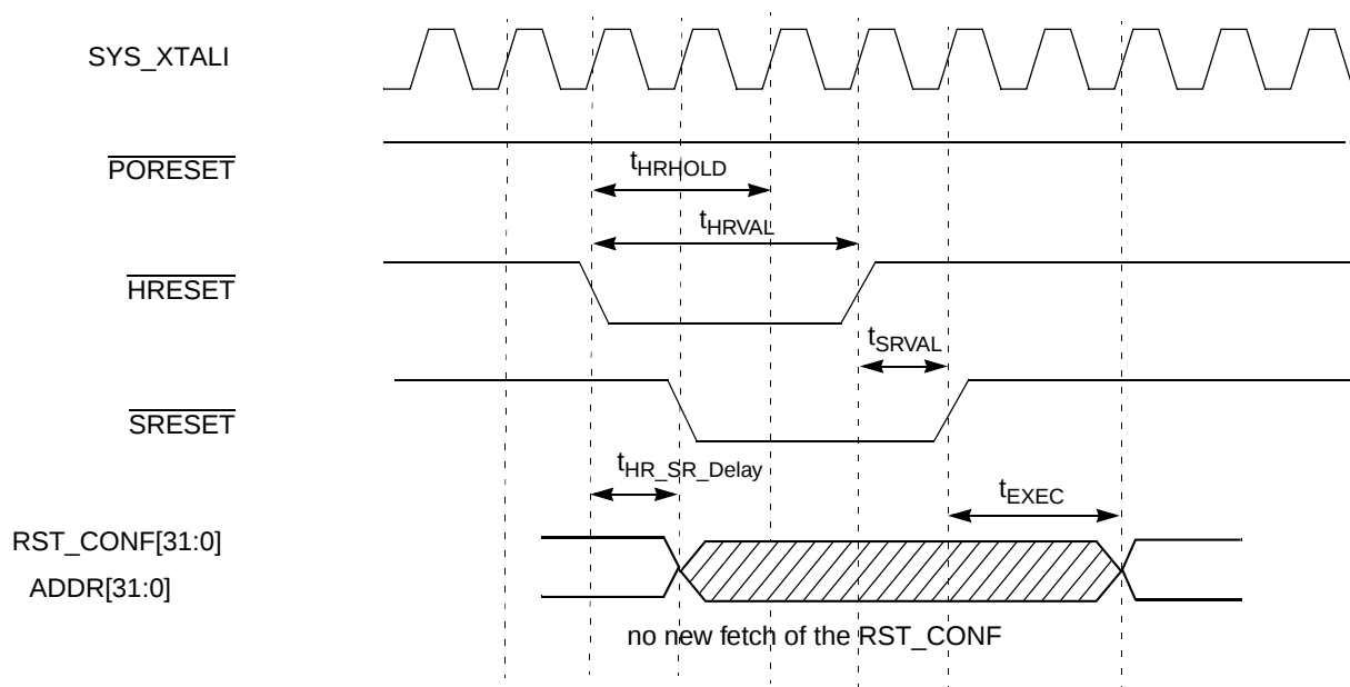
Figure 6. HRESET Behavior
