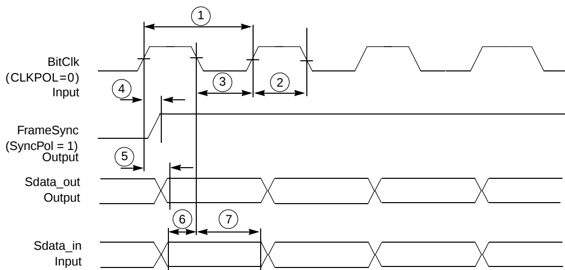
Figure 49. Timing Diagram – AC97 Mode
