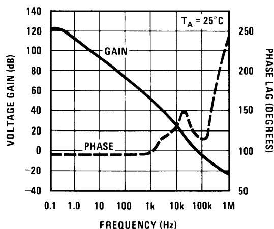
Figure 37. Frequency Response
