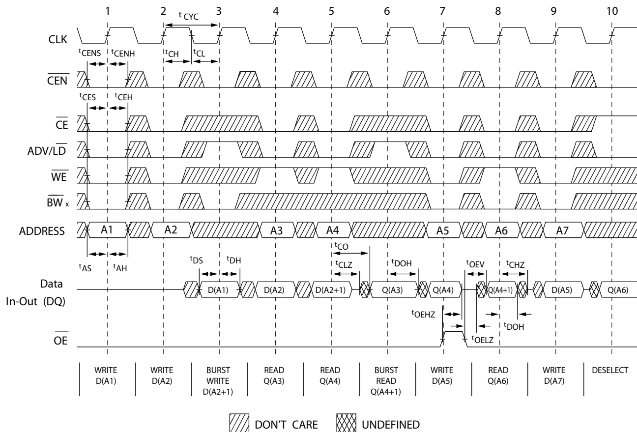
Figure 5. Read/Write/Timing [33, 34, 35]
