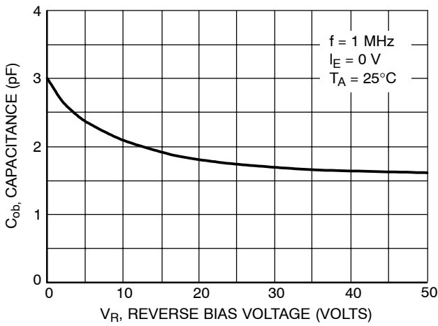
Figure 10. Output Capacitance
