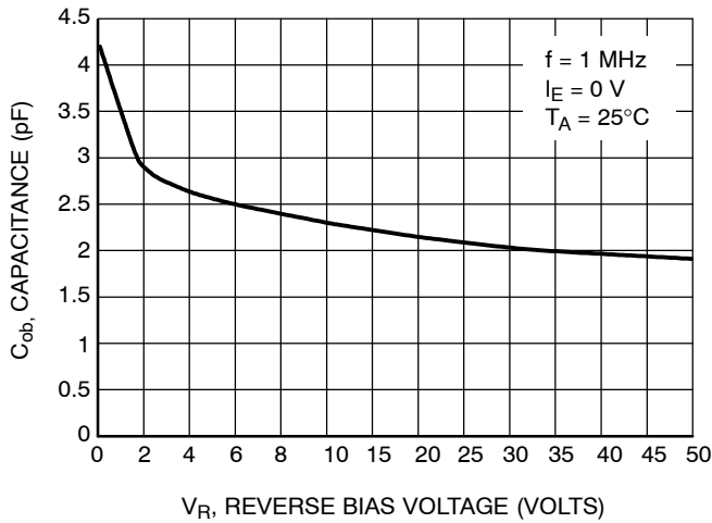
Figure 20. Output Capacitance
