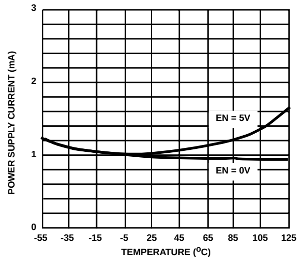
FIGURE 5B. HI-508/HI-509
