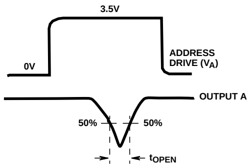
FIGURE 9B. WAVEFORMS
