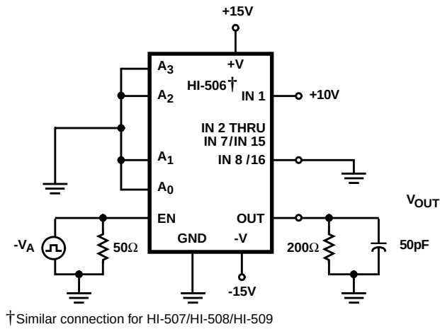
FIGURE 10A. TEST CIRCUIT
