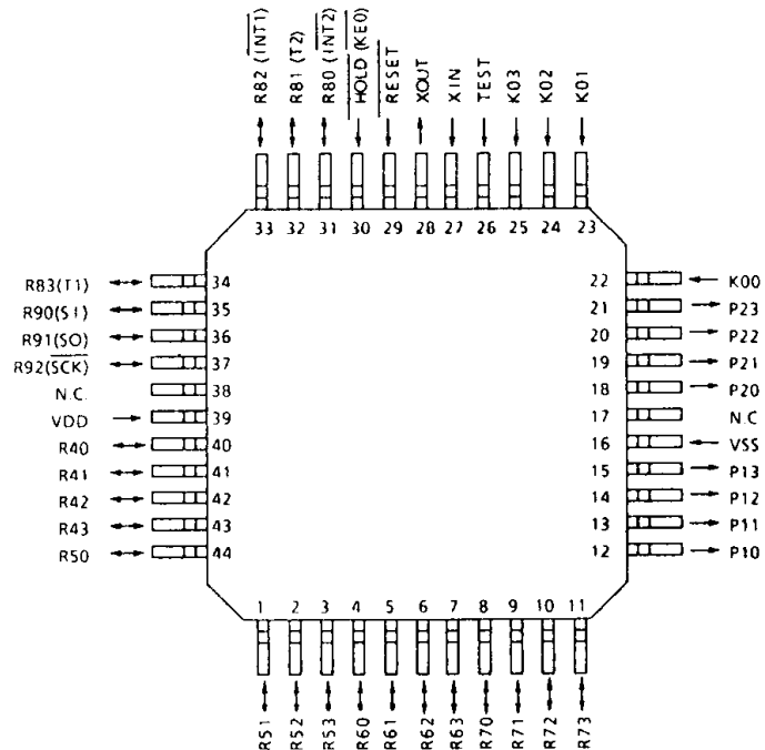
(2) 44-QFP
