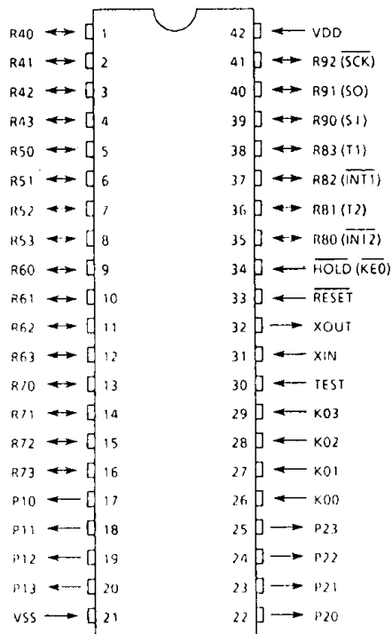
(1) 42-SDIP
