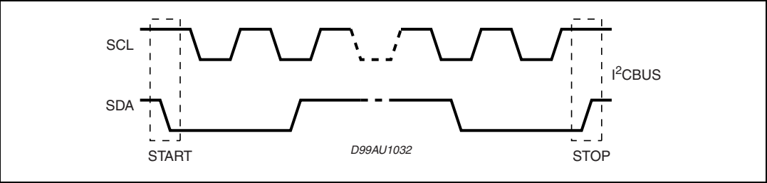
Figure 31. Timing diagram on the I 2 C bus
