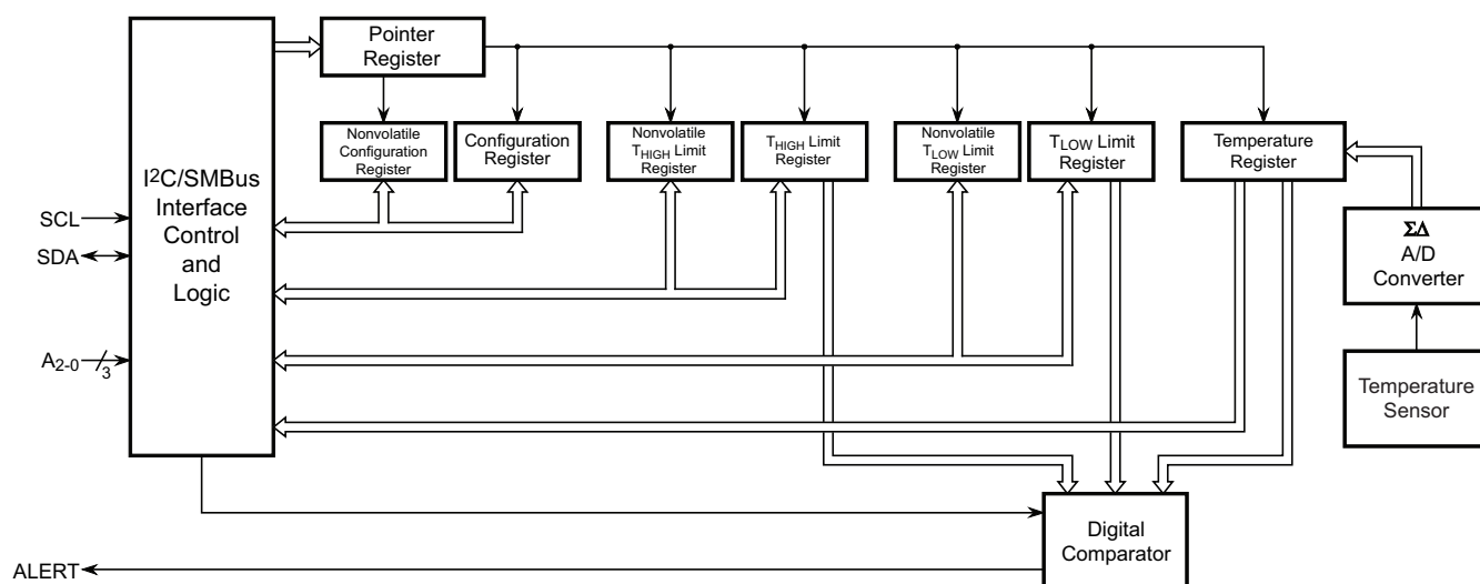
Figure 3-1. Block Diagram
