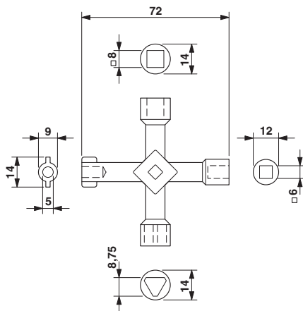
Dimensional drawing
